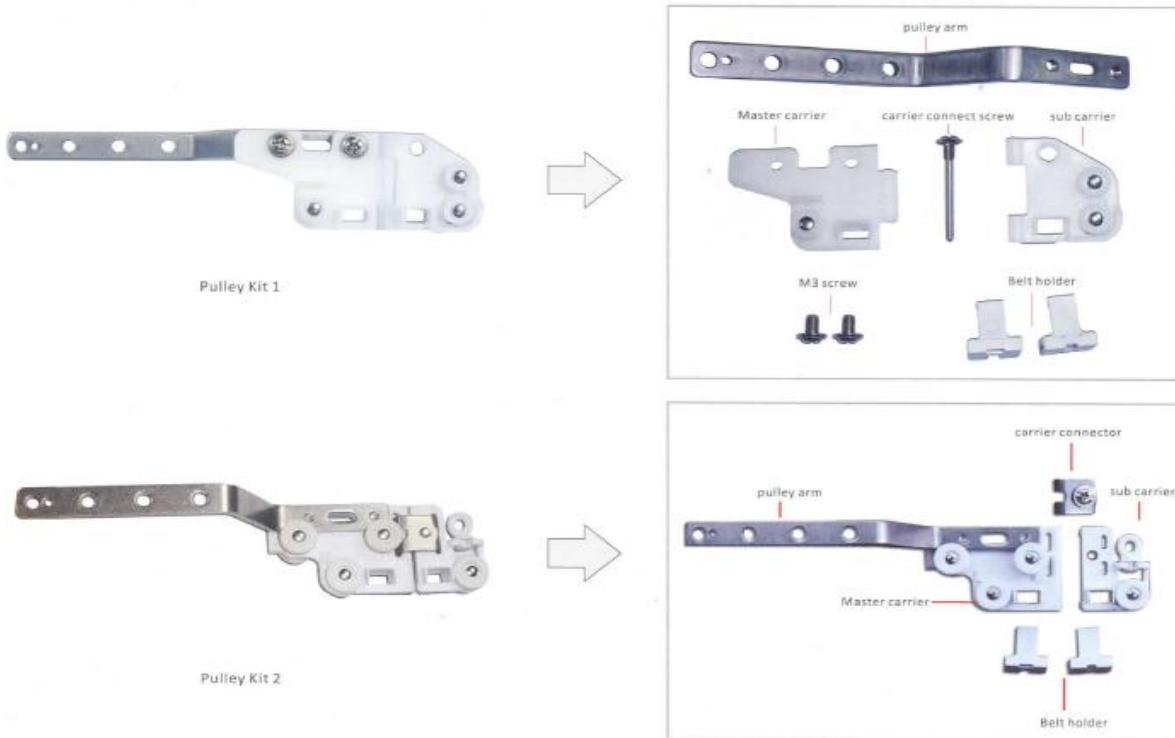
Pulley Diagram
