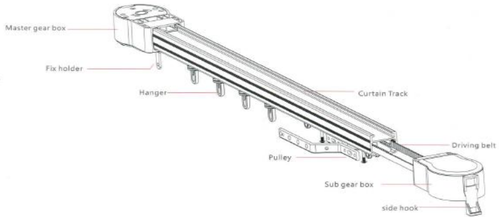
Curtain Motor System Diagram
